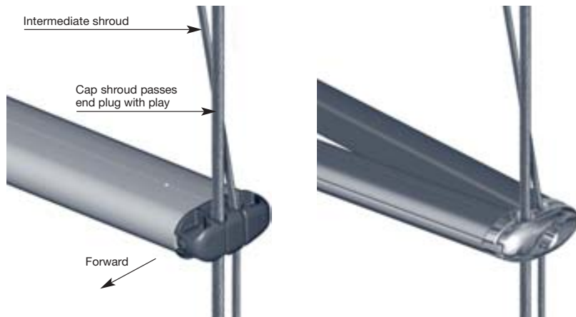
Spreader end plug for continuous rigging.
