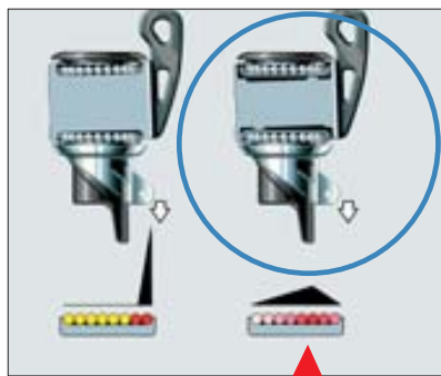
Seldén patented load distributor.
